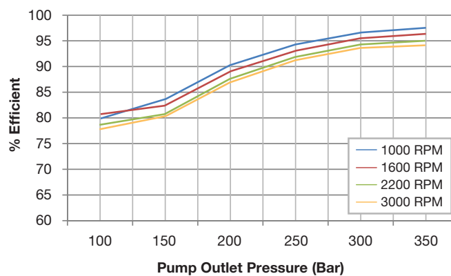
C055 Mechanical Efficiency
