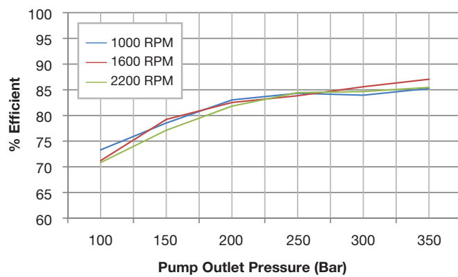
C081 Overall Efficiency
