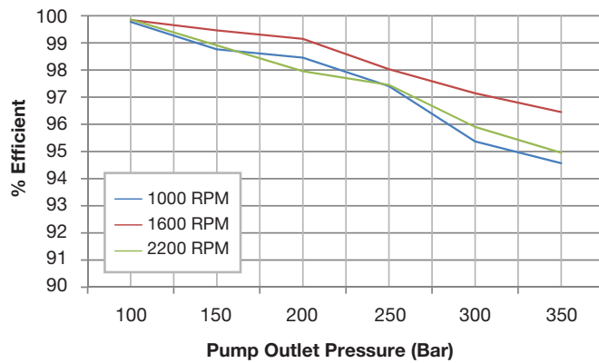
C081 Volumetric Efficiency
