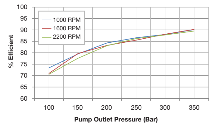
C081 Mechanical Efficiency
