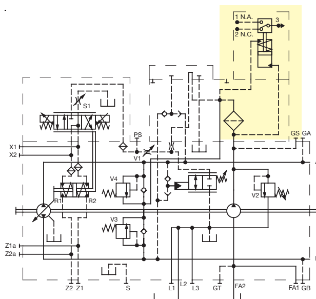
Electrical Sensor
